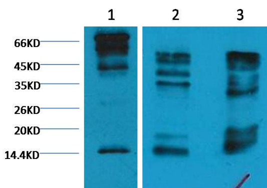
Western blot analysis of 1) Hela, 2) Rat Testis tissue, 3) Raw264.7 with Histone H3 (tri methyl K9) (2C3) Mouse MAb diluted at 1:2000.
