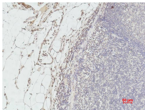
Immunohistochemical analysis of paraffin-embedded Human Colon using Histone H3(tri methyl K9) (TDY127) Mouse mAb diluted at 1:500.
